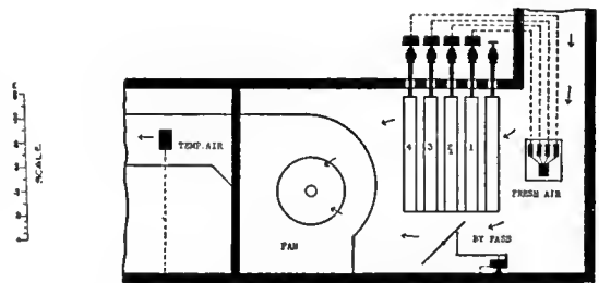
FIG. 5. DIAGRAM SHOWING A COMBINATION OF MULTIPLE AND SINGLE THERMOSTATS IN HOT-BLAST HEATING
